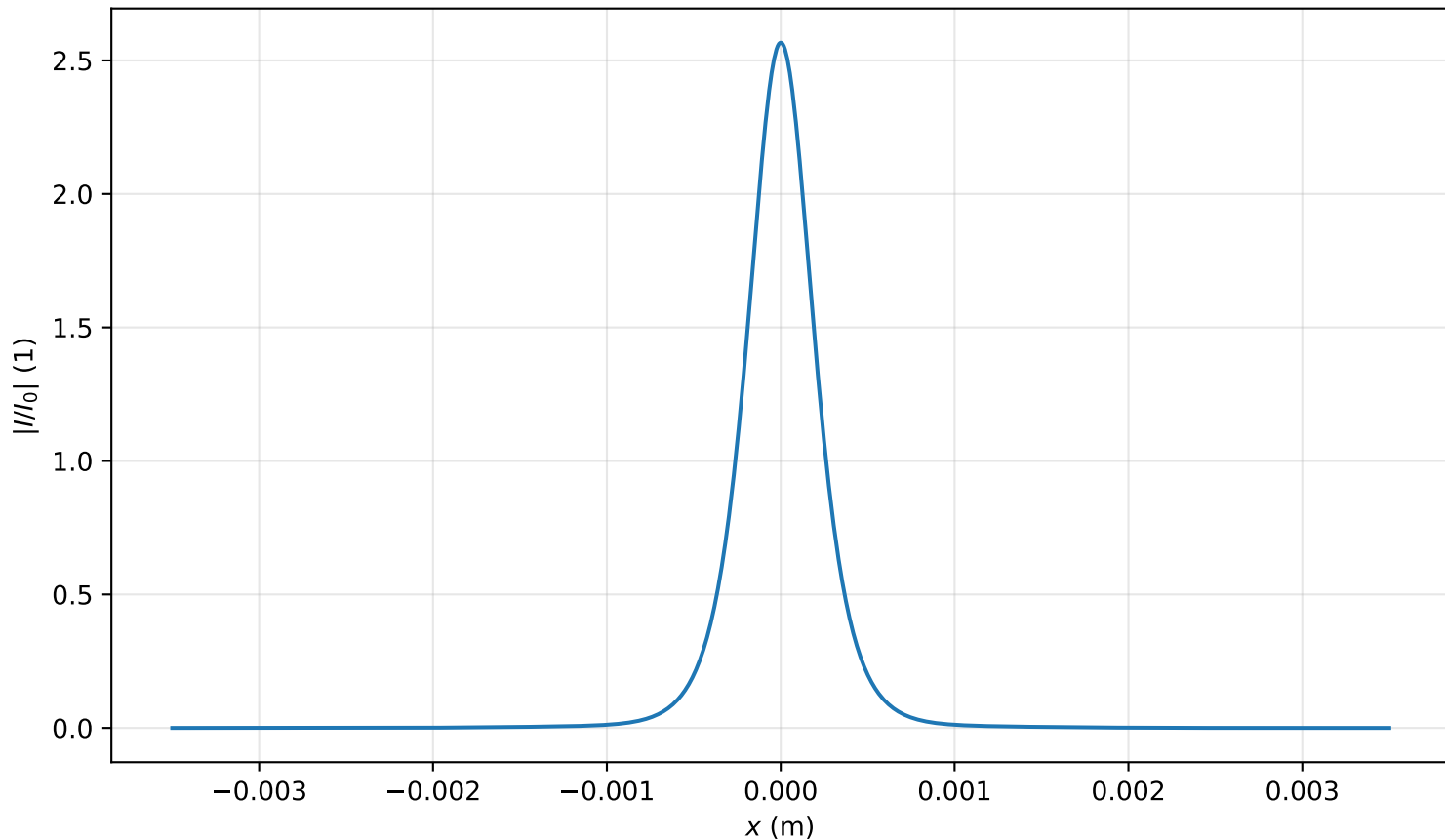
Intensity profile I(x, y = 0, z = 2.866m)/I_0 , P_{in}=1.0P_{cr} , artificial time
